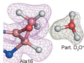
Figure 4. The HYD4 \text{D}_3\text{O}^+ ion hydrogen-bonded to Ala16 in the oxidized rubredoxin structure. The 2F_o - F_c map (contoured at 1\sigma in magenta) is shown, as well as the F_o - F_c omit map ( 3\sigma in green) for which the HYD4 ion was omitted from the structure factor calculation. A \text{D}_3\text{O}^+ ion is also found at the same position in the reduced structure.
