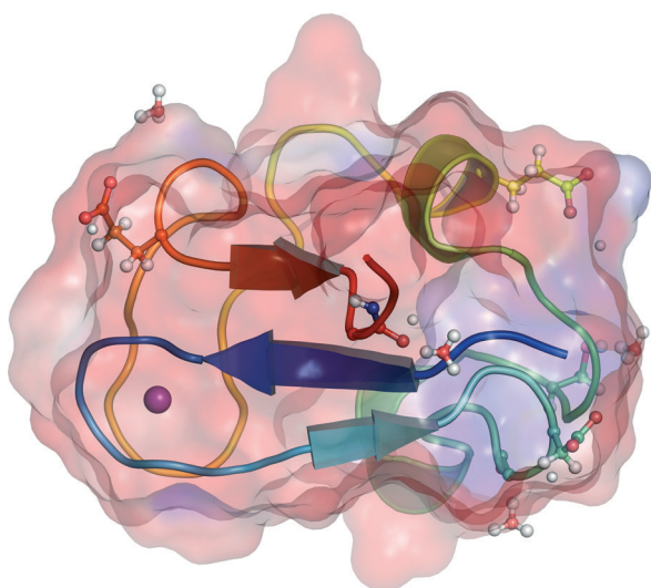
Figure 6. The overall neutron structure of the oxidized form of Pf rubredoxin, showing the D_3O^+ ions (red and gray molecules) and deuterium atoms (gray spheres) bound to carboxylic acid side chains. The electrostatic surface is shown (blue for positive and red for negative).
